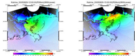
Figure 2. Katrina's storm surge in control run at 12 UTC and 15 UTC 29 August 2005 (ft)
