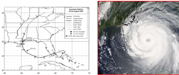
Figure 1. Best track position map prepared by the National Hurricane Center (left) and MODIS-Terra image of Hurricane Katrina (right).
