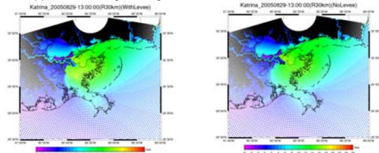
Figure 3. Katrina's storm surge in control run at 13 UTC compared to same simulation without a man-made levee along the Mississippi River up to Chalmette.
