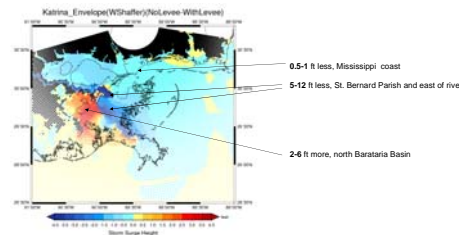
Figure 4. Difference of peak water elevations (No-levee minus levee).
