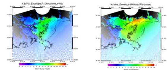
Figure 5. Peak storm surge values for a small (left) and large (right) hurricane with a pressure deficit similar to Katrina..
