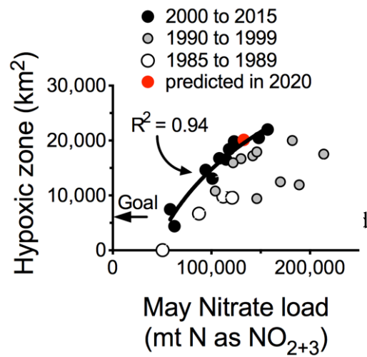
Figure 6. The relationship between nitrate+nitrate in May and the predicted size of the hypoxic zone in July. Several intervals are broken out, with the last one (2000 to 2015) being fit to a regression model. The predicted size of the hypoxic zone for 2020 is indicated by the red dot.
