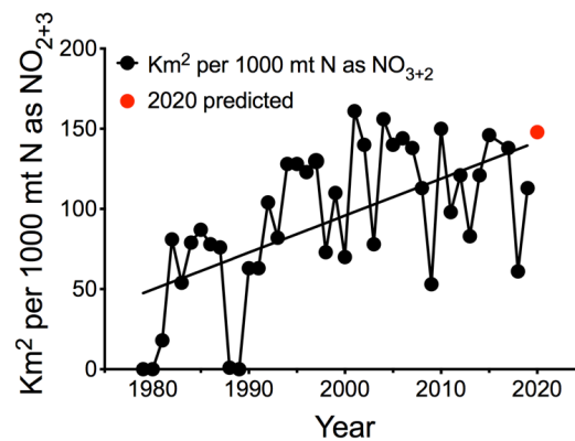
Figure 5. The size of the hypoxic zone per May nitrite+nitrate loading. All years, including strong storm years, are included.
