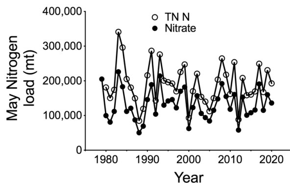
Figure 3. The annual nitrite+nitrate ( \text{NO}_{2+3} ) and total nitrogen (TN) load for the Mississippi River watershed for May. The estimates are from the USGS.
