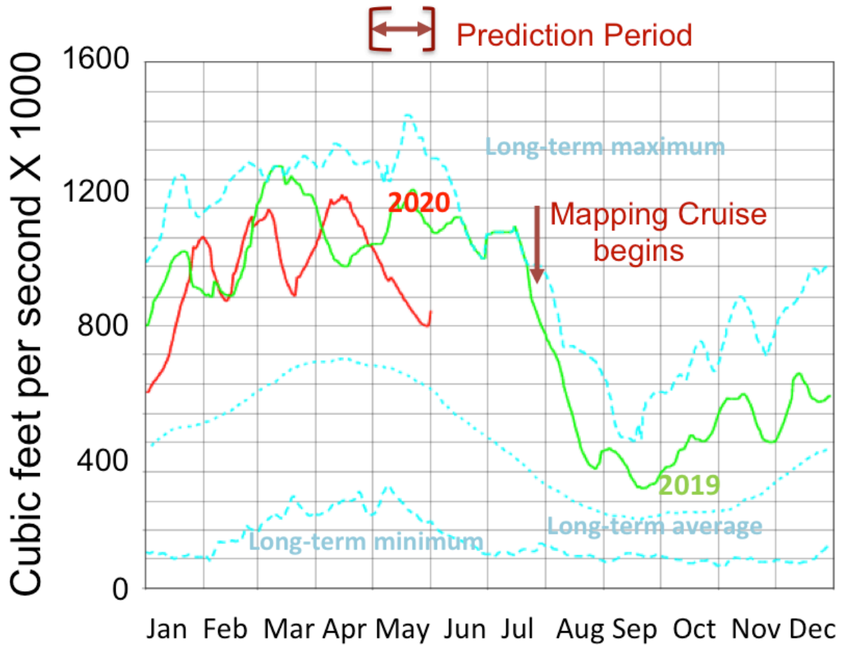
Appendix Figure 3. The daily river discharge at Tarbert Landing, LA, from 1935 through 31 May 2020. Units are cubic feet per second \times 1000. Figure modified from http://rivergages.mvr.usace.army.mil/WaterControl/Districts/MVN/tar.gif .
