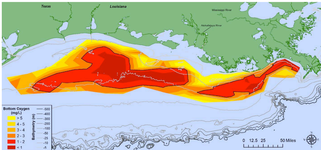
Figure 2. Oxygen concentrations in bottom water across the Louisiana shelf from July 23 – July 30, 2019. Data source: N.N. Rabalais, Louisiana State University, Louisiana Universities Marine Consortium, and R.E. Turner, LSU; funded by NOAA, National Centers for Coastal Ocean Science.
