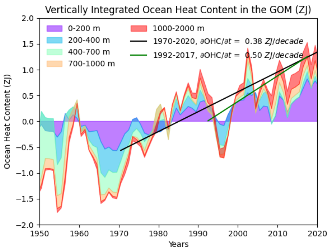
Fig. 6. Vertically integrated ocean heat content between selected layers of the entire GOM from 1950 to 2020 between 0 and 2000m. The anomalies are related to a 1955-2006 (WOA09) baseline. The black line shows the linear regression fitted line based on the OHC in the upper 2000m between 1970 and 2020. While the green line shows the fitted line between 1992 and 2017 to have the same period as ECCO data.
