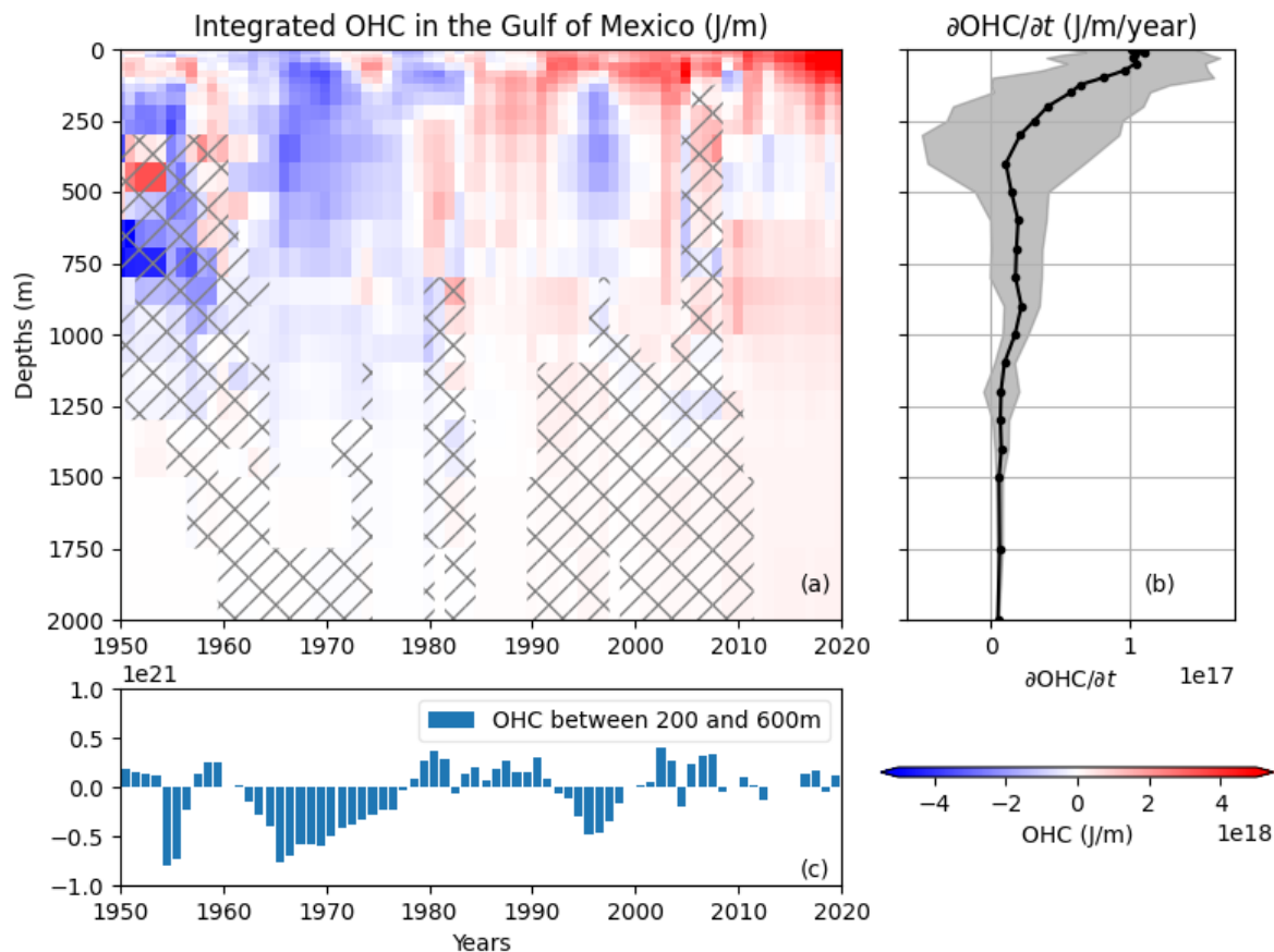
Fig. 4. (a) Spatially integrated OHC in the Gulf of Mexico between 1950 and 2020 as a function of depth (0-2000m) at standard depths. Hatched indicates the data coverage that is less than 30%. (b) The linear trend of OHC change in the GOM at standard depth levels. The rate is divided by the thickness of each layer to make them vertically comparable. The shading area shows the uncertainty of the linear trends (95% confidence intervals). The trend is estimated using linear regression for each standard depth between 1970 and 2020. The trends are statistically significant at all depths ( p -value \leq 0.05 ). Standard depths are defined as 0, 10, 20, 30, 50, 75, 100, 125, 150, 200, 250, 300, 400, 500, 600, 700, 800, 900, 1000, 1100, 1200, 1300, 1400, 1500, 1750, 2000m. Anomalies are relative to a 1955-2006 baseline. (c) Vertically integrated OHC between 200 and 600m.
