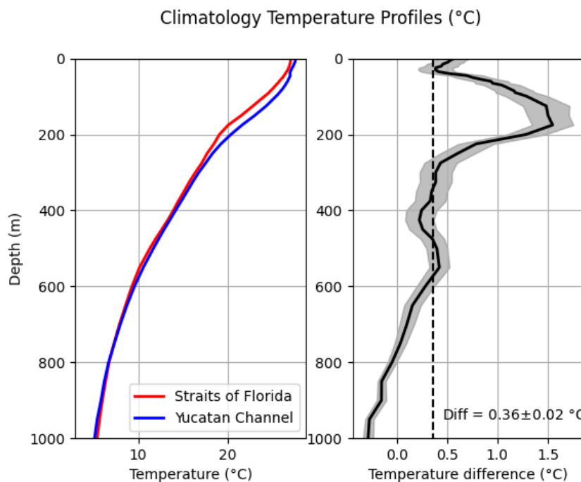
Fig. 7 (a) Climatology mean temperature profiles at Straits of Florida and Yucatán Channel in the upper 1000m. (b) The temperature difference between the Yucatán Channel and the Straits of Florida. The shaded area shows \pm 1 standard deviation (std). The dashed vertical is the vertical mean of the temperature difference. 0.1^\circ \times 0.1^\circ regional climatological temperature fields for the GOM ( https://www.ncei.noaa.gov/products/gulf-mexico-regional-climatology ) are used. The profile for Straits of Florida is averaged from all profiles within an
