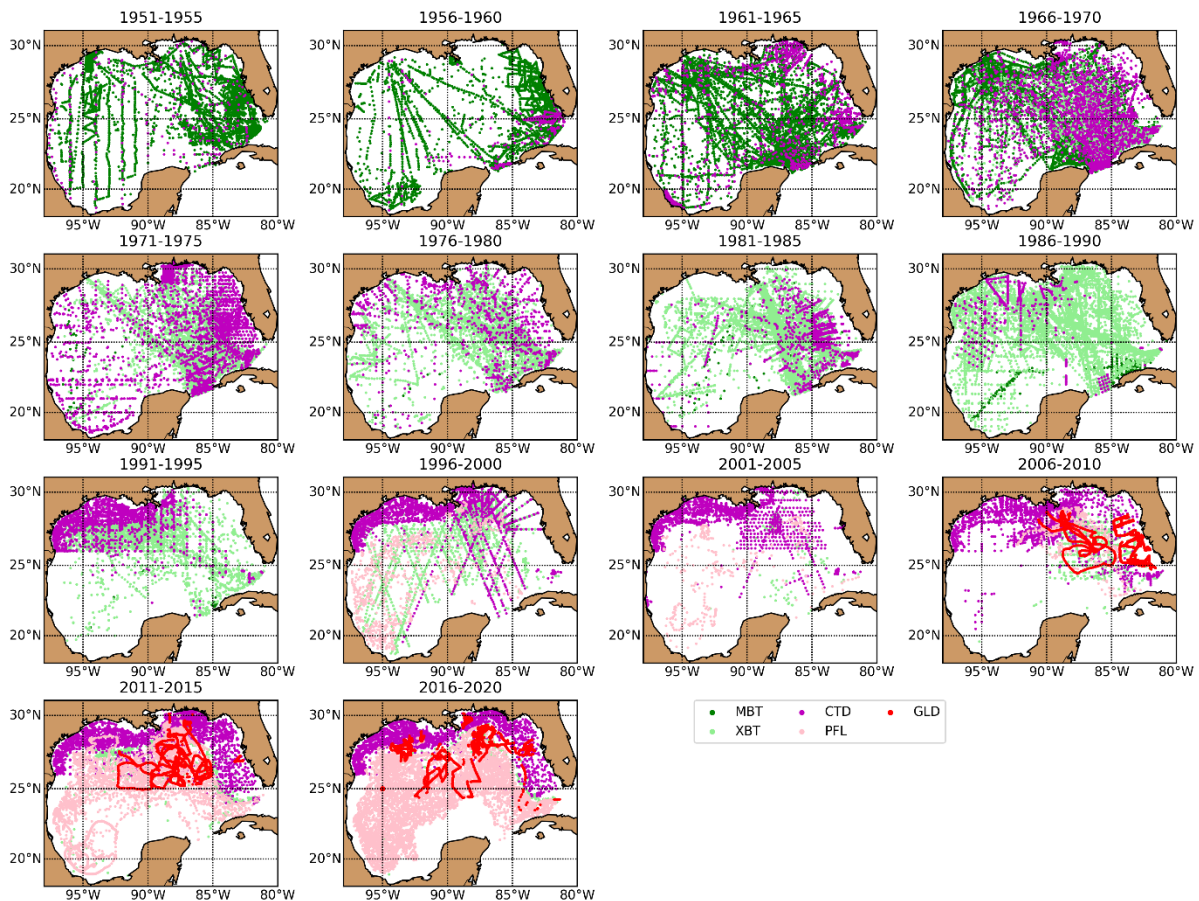
Fig. 1. Temperature profiles' spatial distribution for every pentadal (5-year) period from 1951 to 2020. The color shows different measurement types. MBT: mechanical bathythermograph (MBT) data, digital BT (DBT), and micro-BT ( \mu BT); XBT: expendable bathythermograph and AXBT; CTD: bottle, Conductivity-Temperature-Depth (CTD), expendable CTD (XCTD) data; GLD: glider data; PFL: profiling float data, mainly from the Argo program. Some of the data points may not be shown due to data overlap.
