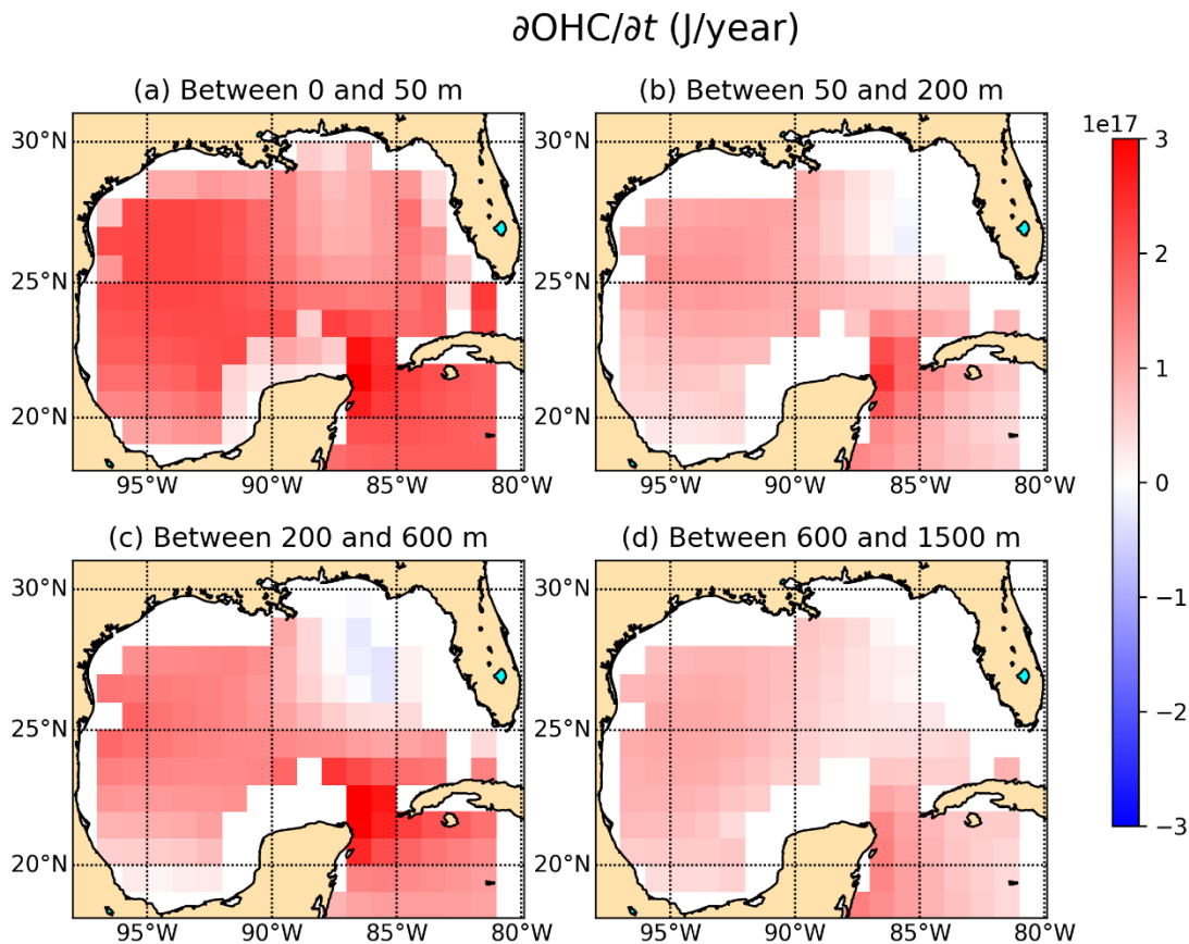
Fig. 5. Spatial distribution of the OHC change with time (units: J/year) between different layers (a) 0-50m; (b) 50-200m; (c) 200-600m; and (d) 600-1500m. The OHC trends are estimated using linear regression between 1970 and 2020 at each grid point between different depth layers.
