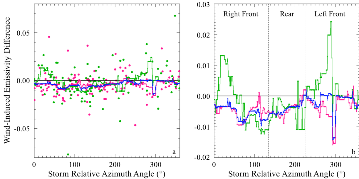
Figure 6. Wind-induced emissivity difference versus azimuth angle for the \geq 20 \text{ms}^{-1} wind speed range separated by radii \leq 50 km (green) and radii > 50 km (pink). The solid lines are the running medians for 30° azimuthal bins and the blue line is for all of the \geq 20 \text{ms}^{-1} wind speed range data. The storm relative sectors are noted in (b) by the vertical dashed black lines and respective labels.
